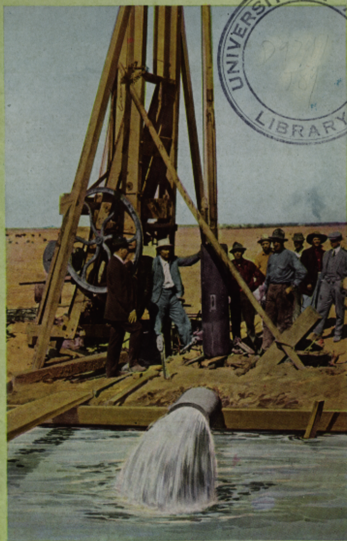
BRINGING IN A WELL FLOWING 1,000 GALLONS PER MINUTE
